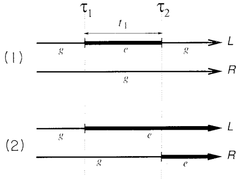
FIG. 2. Double-sided Feynman diagrams in second order. The lines denoted by L and R represent the time evolution of the left- (ket) and the right- (bra) hand sides of the density matrix, respectively. The thin and thick lines denote the ground state |g\rangle and the excited state |e\rangle . Path 1 corresponds the transition from g to g , whereas path 2 corresponds the transition from g to e . Two other paths, which are the Hermitian conjugates of the above paths, are not shown. These conjugate paths can be obtained by interchanging L and R .
