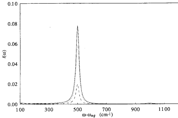
FIG. 4. Absorption spectrum [Eq. (5.19)] with Condon and non-Condon dipole interactions for a weak damping case, \gamma = 0.05\omega_0 . The fundamental 0-0 transition (not shown) is 230 times more intense. The solid line ( \mu' = 0.1, \mu'' = 0.01 ) indicates the non-Condon interaction, whereas the dashed line indicates the Condon approximation. The difference between these two lines is shown by the dotted line.
