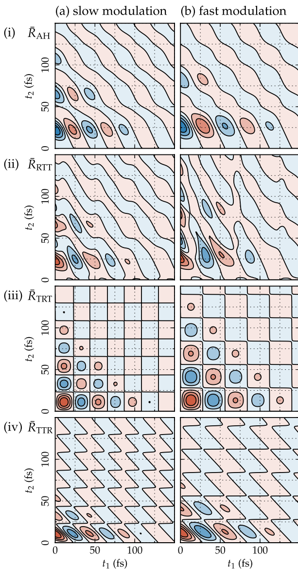
FIG. 12. The 2D profiles of the (i) \bar{R}_{\text{AH}} , (ii) \bar{R}_{\text{RTT}} , (iii) \bar{R}_{\text{TRT}} , and (iv) \bar{R}_{\text{TTR}} components for the (a) slow modulation ( \zeta = 1.5 \omega_0 and \gamma = 0.5 \omega_0 ) and (b) fast modulation ( \zeta = 0.2 \omega_0 and \gamma = \infty ) cases obtained from the anharmonic ( g_3 = 0.1 ) LL BO model. Contours in red and blue represent positive and negative values, respectively.
