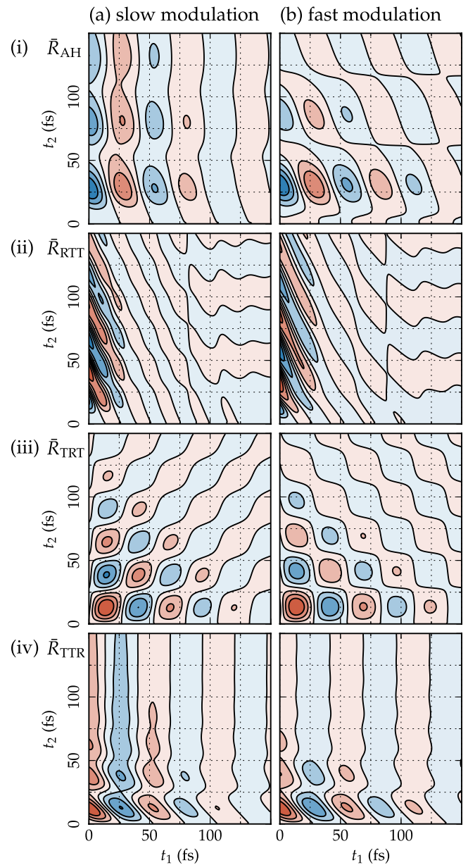
FIG. 13. The 2D profiles of the (i) \bar{R}_{\text{AH}} , (ii) \bar{R}_{\text{RTT}} , (iii) \bar{R}_{\text{TRT}} , and (iv) \bar{R}_{\text{TTR}} components for the (a) slow ( \zeta = \omega_0 and \gamma = 0.5 \omega_0 ) and (b) fast modulation ( \zeta = 0.49 \omega_0 and \gamma = \infty ) cases obtained from the anharmonic ( g_3 = 0.1 ) SL BO model. Contours in red and blue represent positive and negative values, respectively.
